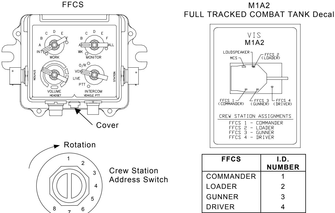
Figure 3-1. FFCS Crew Station Address Switch
